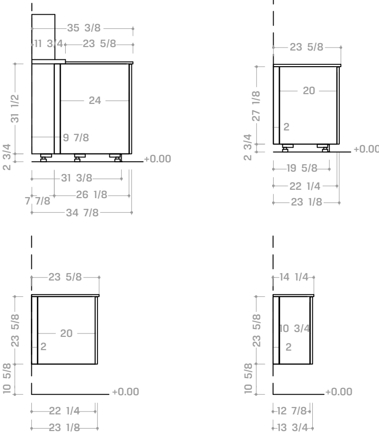
Base module with Medley type A-B shelf
