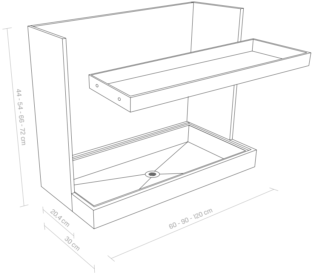
Scaffale Medley con vasca sifonata. Medley shelving unit with draining section complete with siphon.
