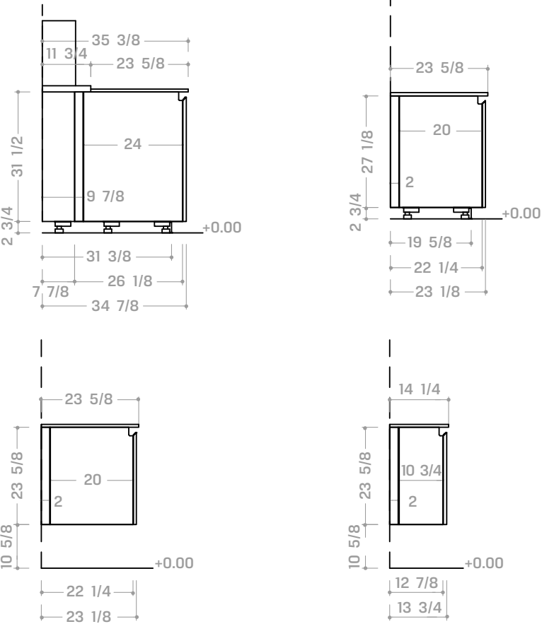
Base module with Medley type A-B shelf
